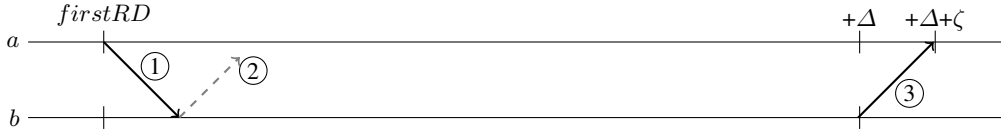
Fig. 1. Reasons why a node waits \Delta + \zeta for receiving potential affiliation messages. First of all, note that information messages cannot be lost when they are sent on an appearing edge, neither can their potential affiliation answer, because of the assumption that edges appears at least for 2 \times \zeta time units. The loss of such messages can only occur when the information is directly relayed by a node who received it (say, node a , relaying at time firstRD the information to node b ). If the information message is lost, then this is not a problem (it simply means that this edge at that time did not have to be used). If the affiliation message is lost, however, it must be sent again. In the worst case, the common edge disappears just before the affiliation message is delivered, and reappears only \Delta - 2 \times \zeta later (see Property 1). Affiliation messages can thus be received until firstRD + \Delta + \zeta .
